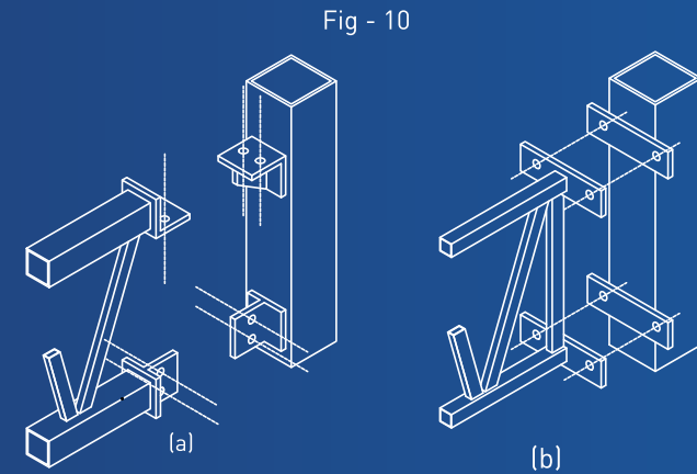
Figure 10(a&b) - Truss to SHS/RHS column connection
