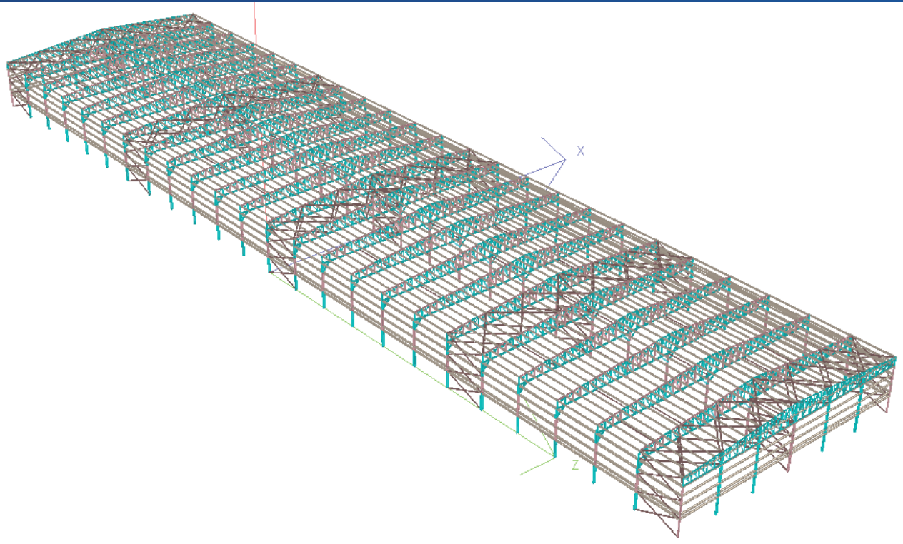
ISOMETRIC VIEW
